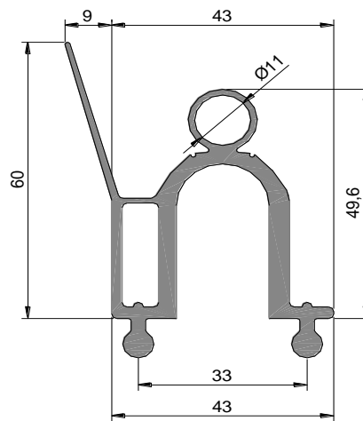
Drawing OSE-P 45 60 04
